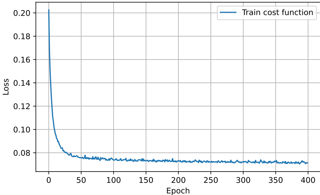
Cost on the training set
